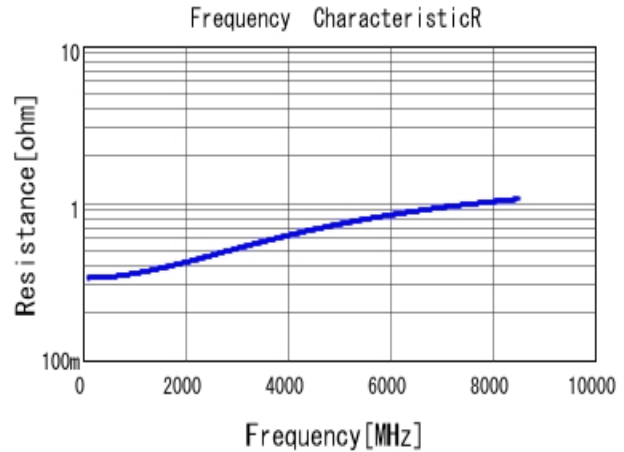
■ GRM0335C1H1R3CA01 R DC0V, 25degC
