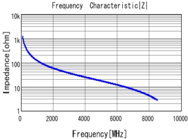
■ GRM0335C1H1R3CA01 |Z| DC0V, 25degC
