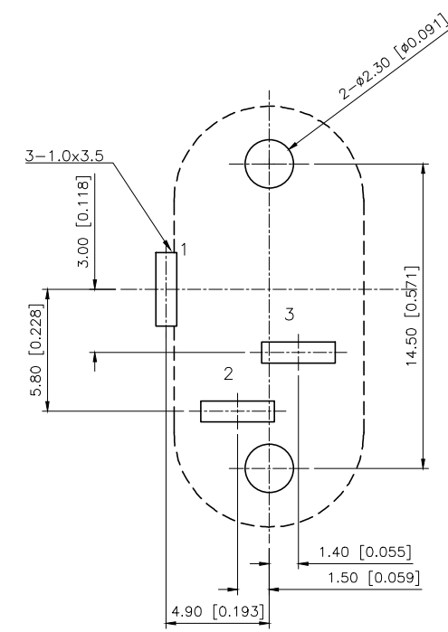
PCB LAYOUT FRONT VIEW
