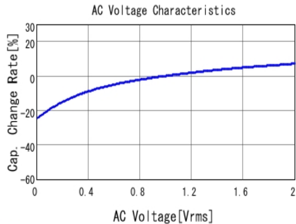
■ GRM188Z71E225KE43 C-AC Voltage capchange, DC0V, 25.0d
