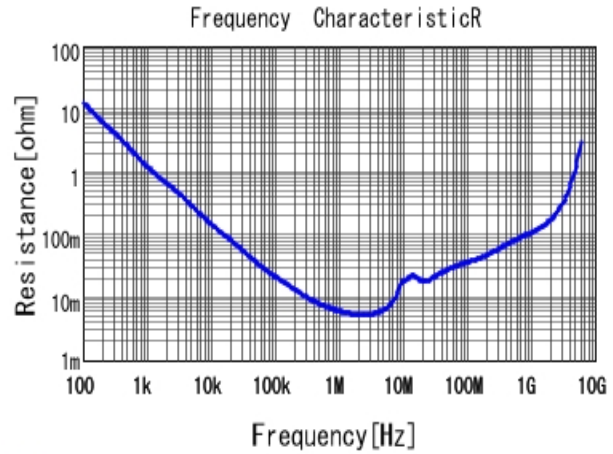
■ GRM188Z71E225KE43 R DC0V, 25degC
