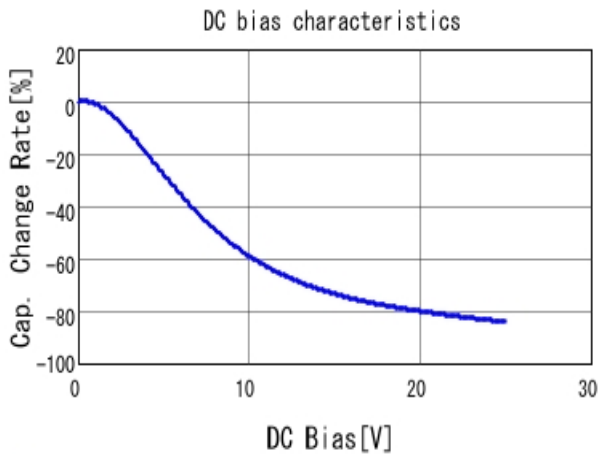
■ GRM188Z71E225KE43 C-DC bias capchange, 25.0degC, AC1V
