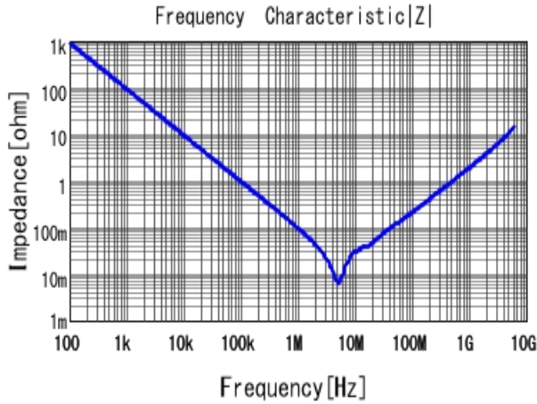
■ GRM188Z71E225KE43 |Z| DC0V, 25degC
