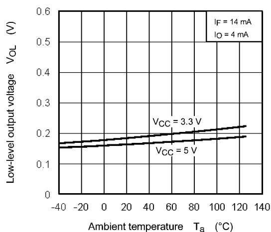
Fig. 12.2.3 V_{OL} - T_a
