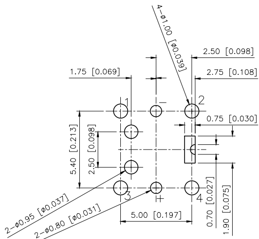
PCB LAYOUT
