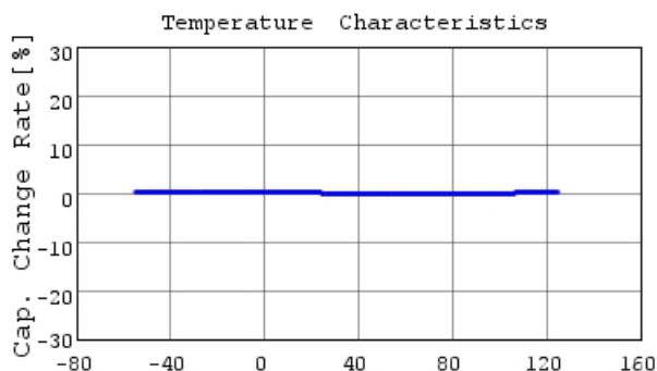
GRM2165C1H333GA01 C-Temp. capchange, DCOV, 1
