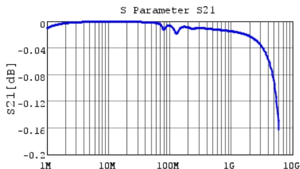
GRM2165C1H333GA01 S21 DCOV, 25degC
