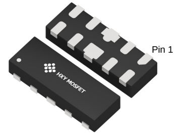
DFN2510-10L (DFN2510D-10))
