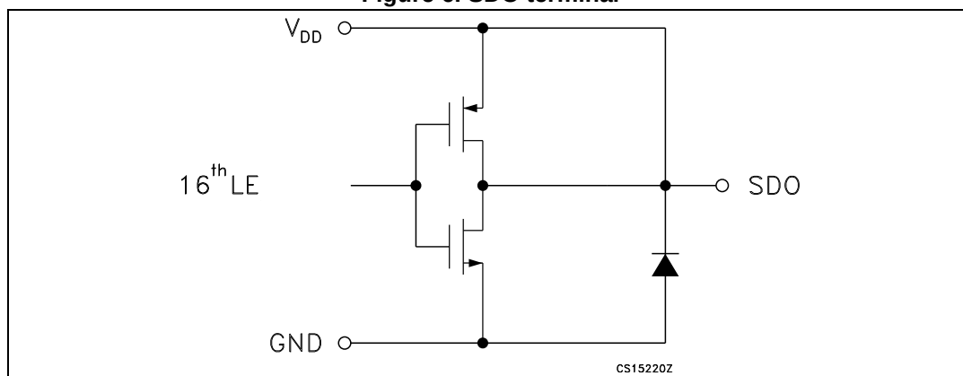
Figure 6. SDO terminal
