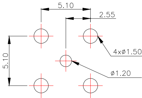
PCB.WELDING DRAWING (TOLERANCE:±0.05)
