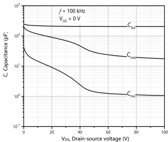
Figure 3, Typ. capacitances
