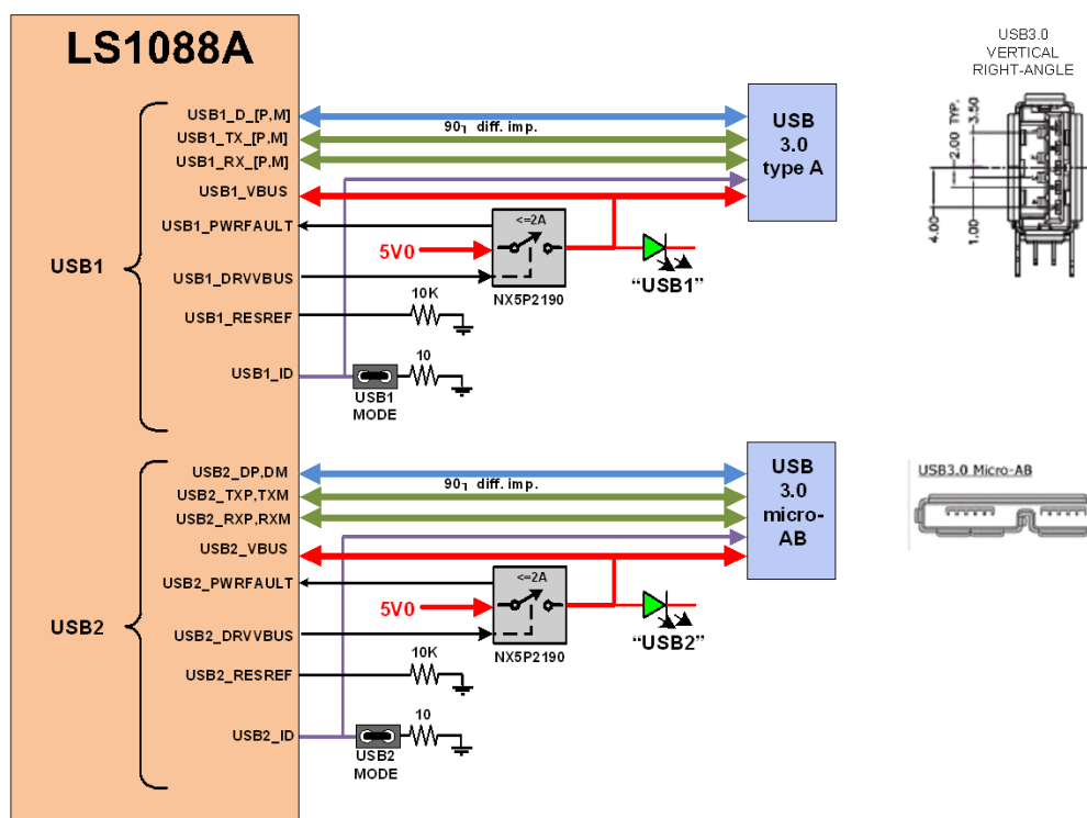
Figure 2-14. USB architecture
