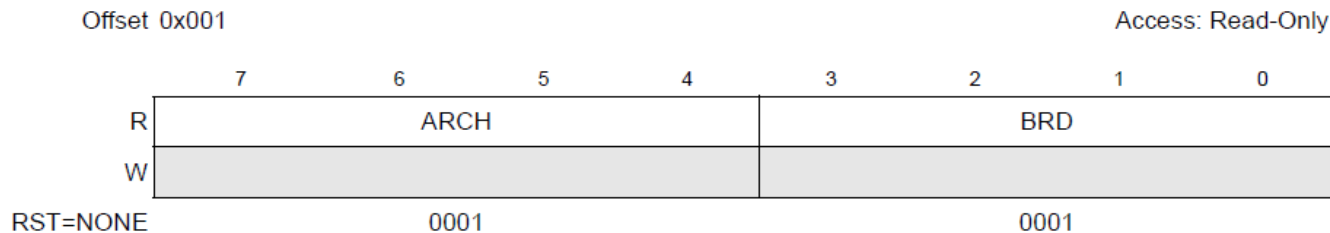
Figure 3-2. VER Register
