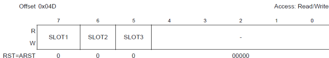
Figure 3-31. RST_MASK3 Register
