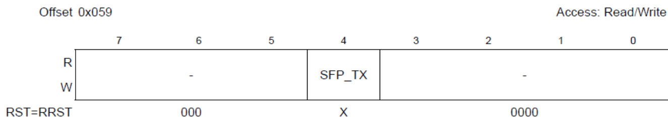
Figure 3-37. BRDCFG9 Register
