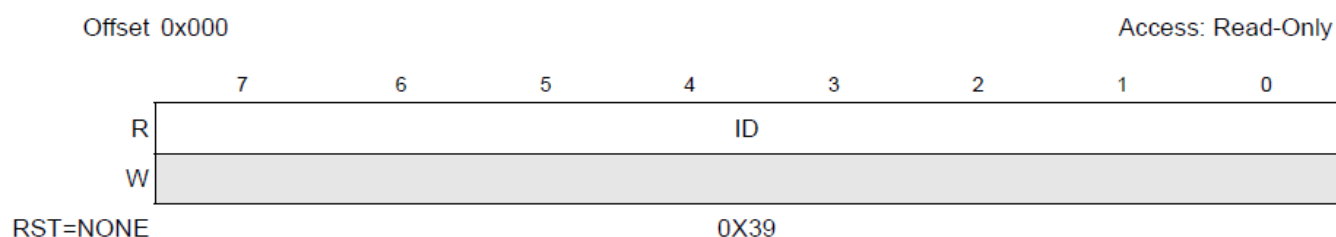
Figure 3-1. ID Register
