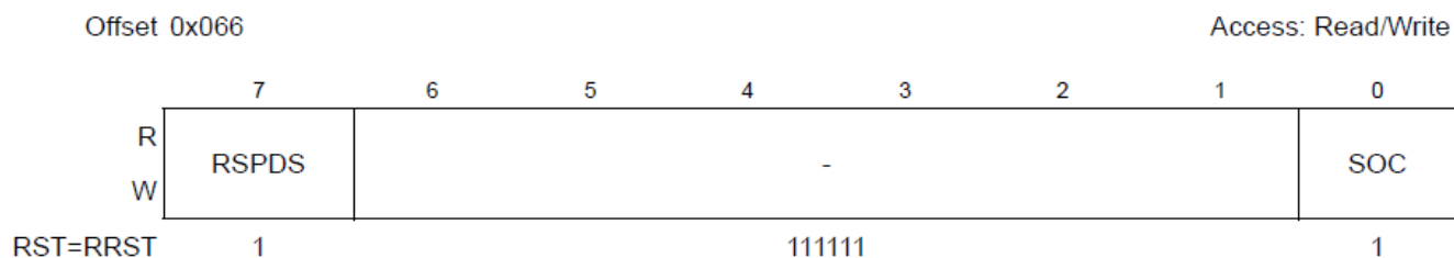
Figure 3-41. DUTCFG6 Register
