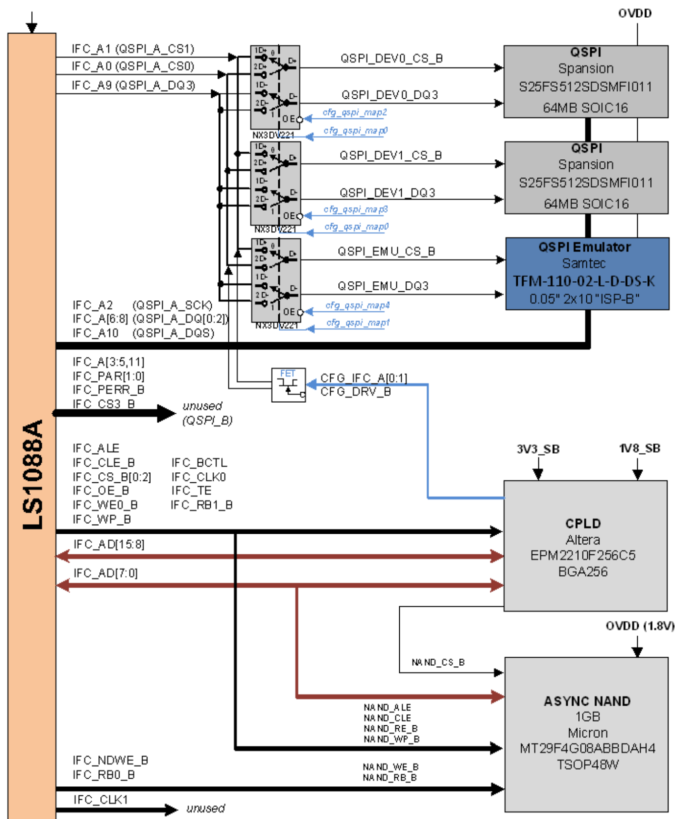
Figure 2-10. IFC interface
