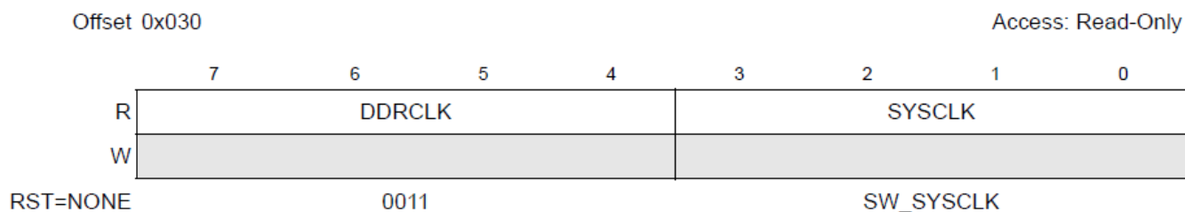
Figure 3-19. CLK_SPD1 Register
