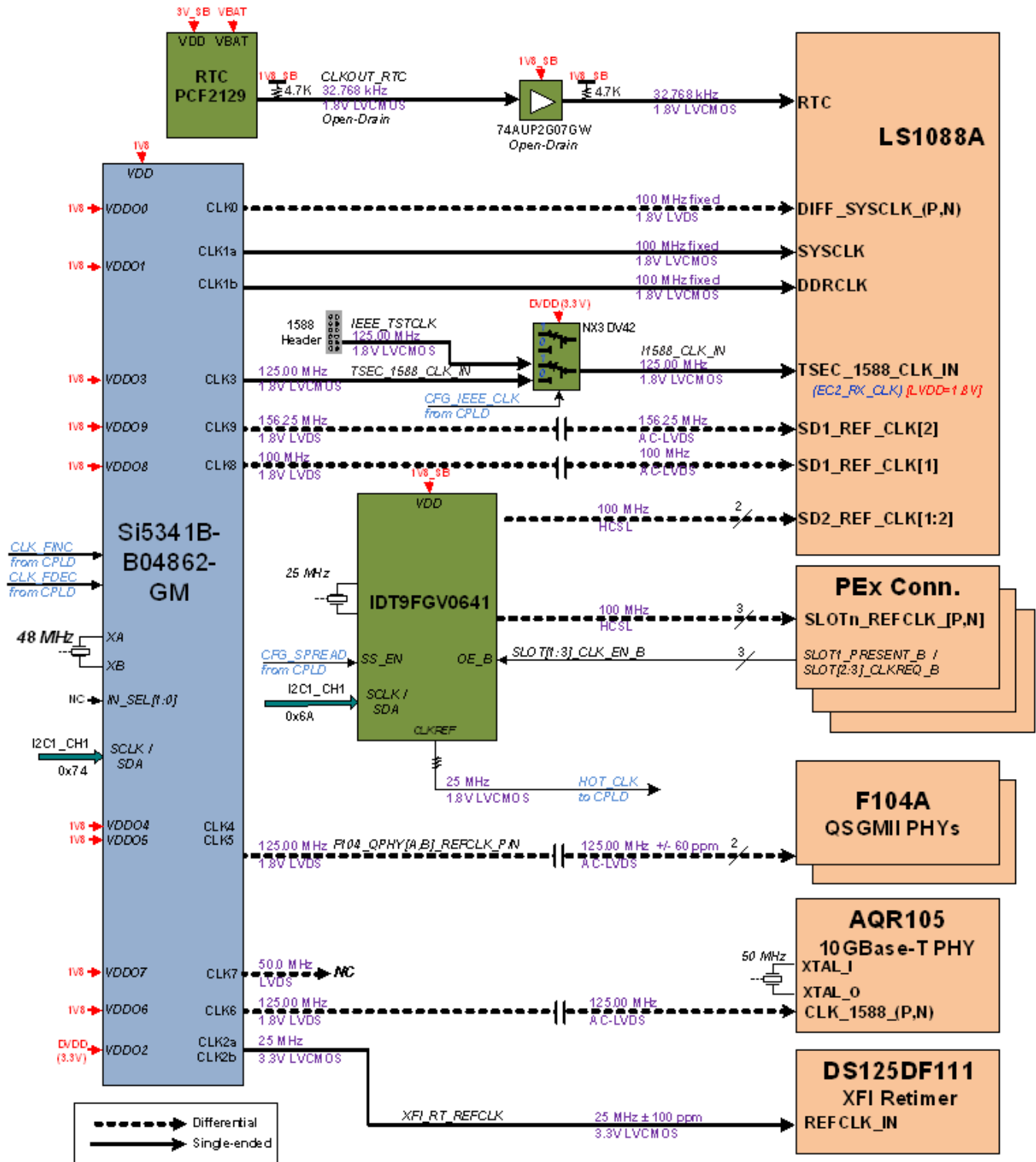
Figure 2-5. Clock architecture
