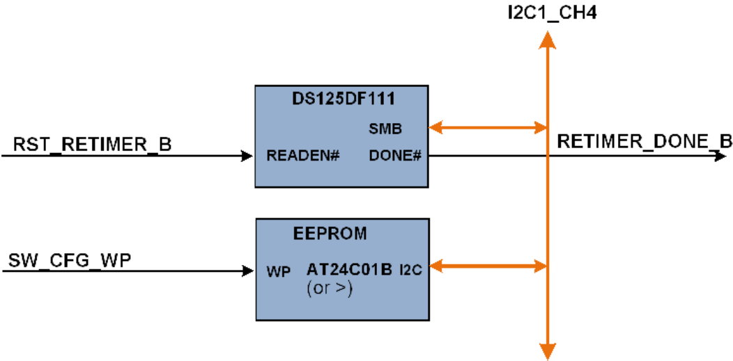
Figure 2-8. Retimer Self-Initialization
