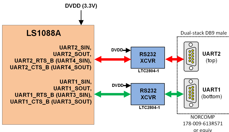
Figure 2-23. DUART interfaces
