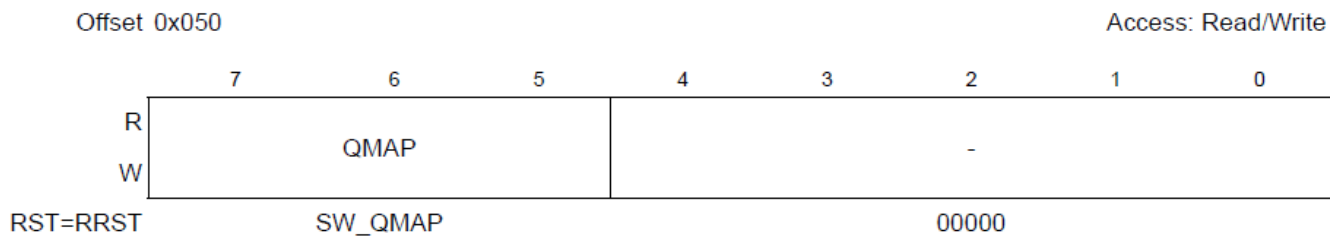
Figure 3-32. BRDCFG0 Register
