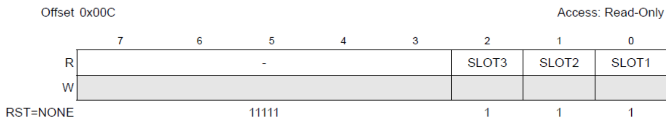
Figure 3-11. STAT_PRES2 Register
