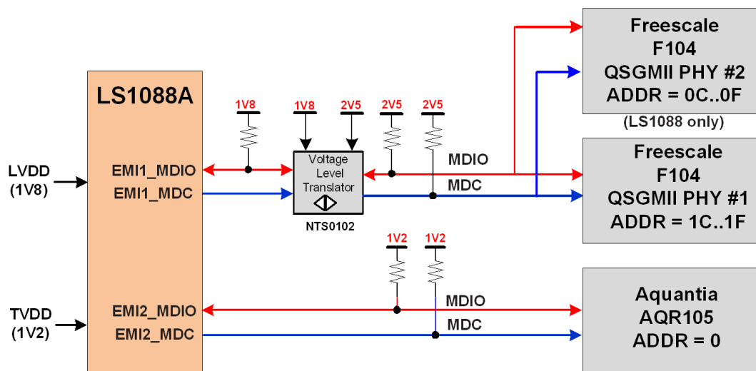
Figure 2-9. EMI interfaces
