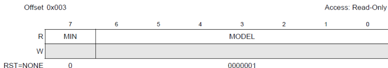
Figure 3-4. MODEL Register
