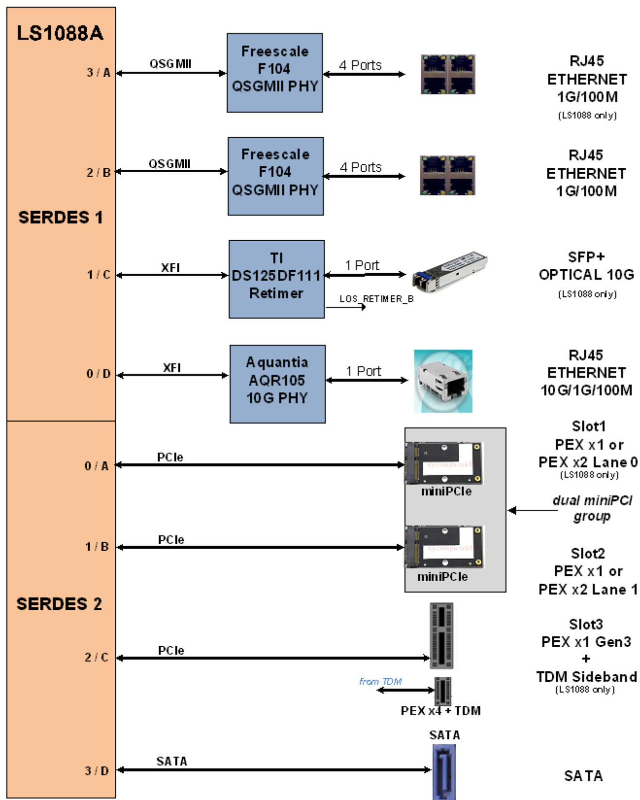
Figure 2-7. SerDes connectivity
