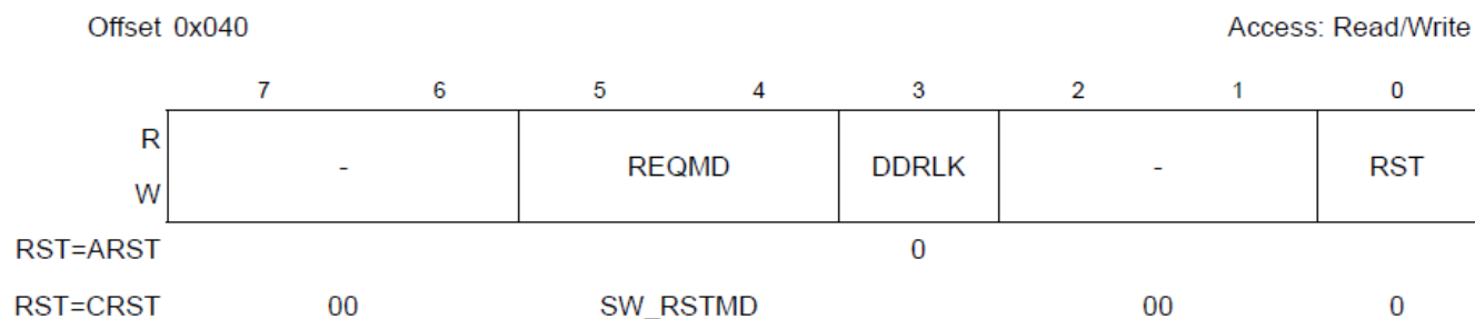
Figure 3-23. RST_CTL Register
