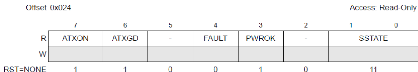
Figure 3-16. PWR_MSTAT Register
