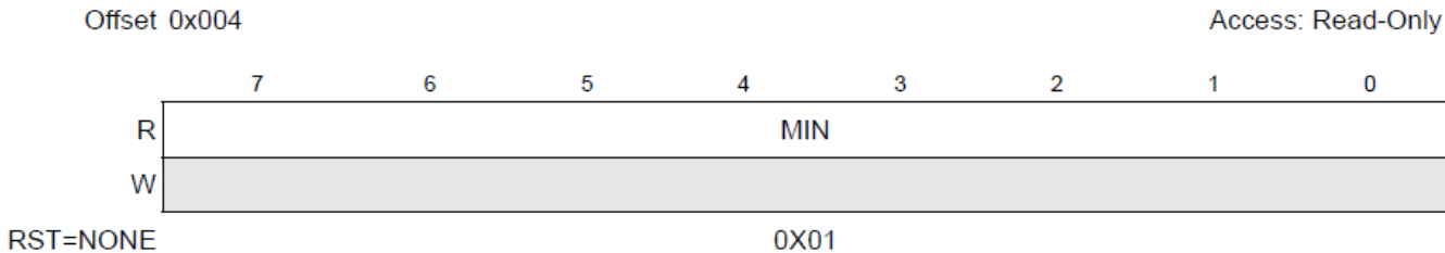
Figure 3-5. MINOR Register
