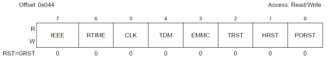
Figure 3-27. RST_FORCE2 Register
