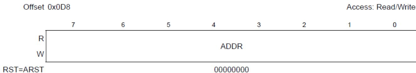
Figure 3-44. CMSA Register
