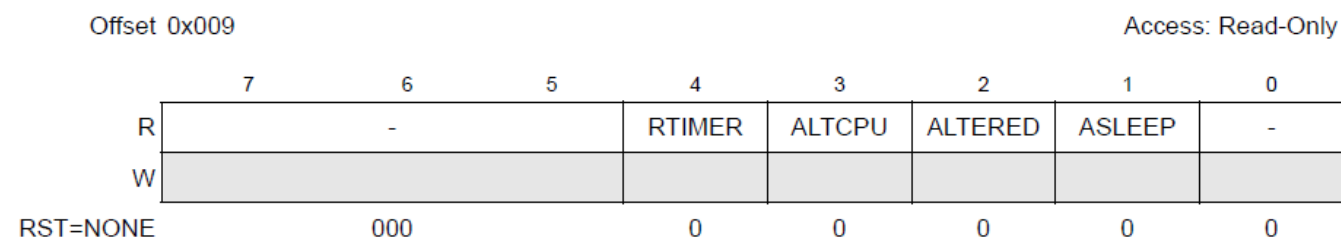
Figure 3-8. STAT_SYS Register
