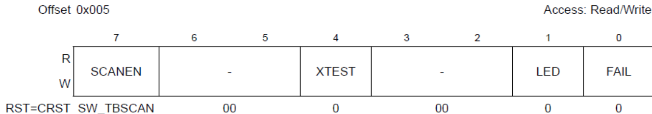
Figure 3-6. CTL Register
