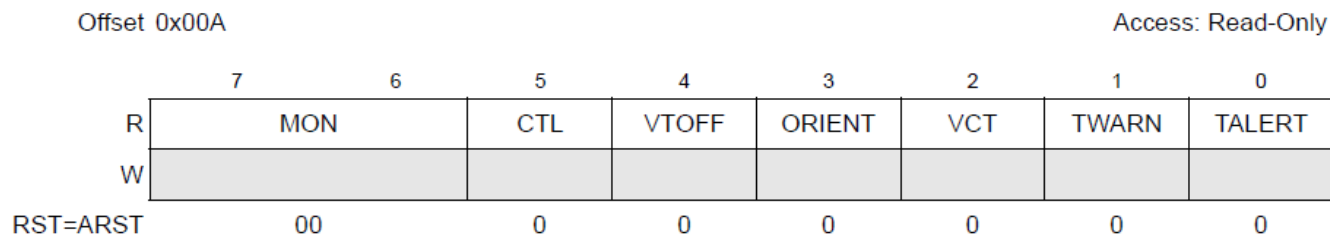
Figure 3-9. ALARM Register
