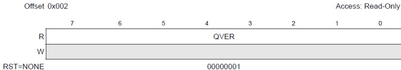
Figure 3-3. QVER Register
