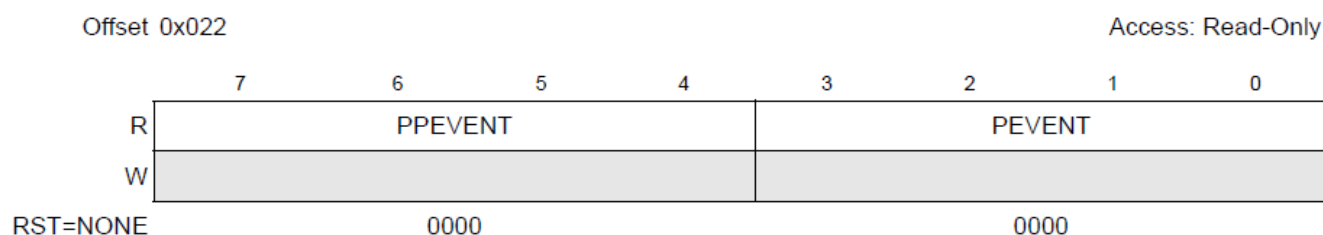
Figure 3-15. PWR_EVENT Register
