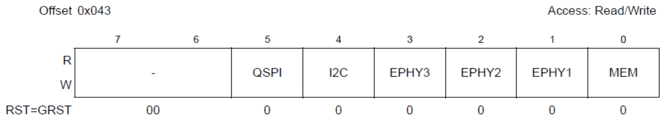
Figure 3-26. RST_FORCE1 Register
