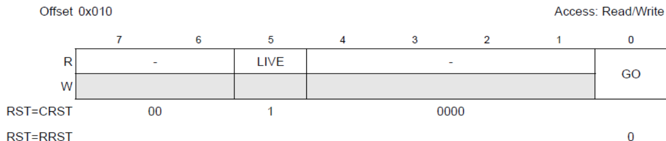
Figure 3-13. RCFG Register
