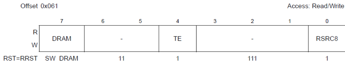
Figure 3-39. DUTCFG1 Register
