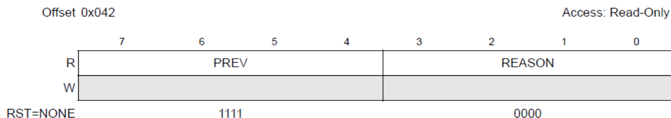
Figure 3-25. RST_REASON Register
