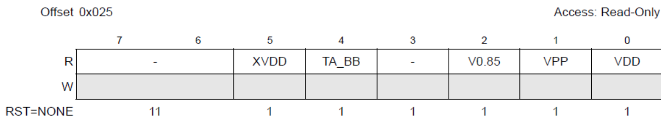
Figure 3-17. PWR_STAT1 Register
