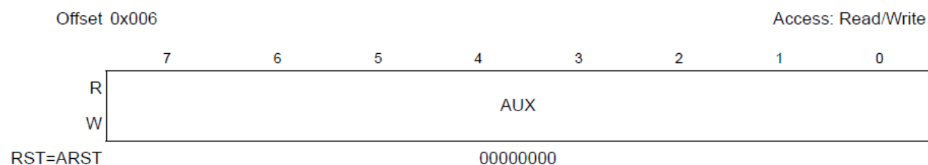
Figure 3-7. AUX Register
