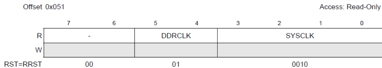
Figure 3-33. BRDCFG1 Register
