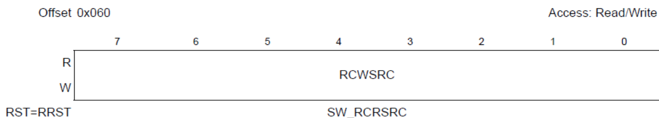
Figure 3-38. DUTCFG0 Register
