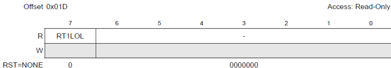
Figure 3-14. LOS_STAT Register
