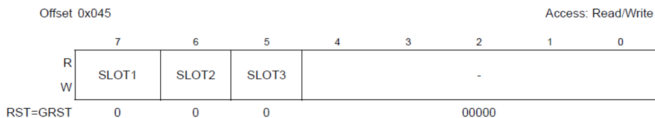
Figure 3-28. RST_FORCE3 Register
