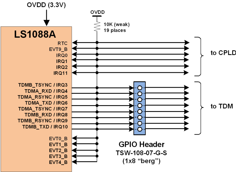
Figure 2-17. Interrupt Architecture
