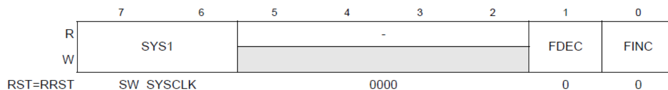
Figure 3-22. SYSCLK_D1 Register
