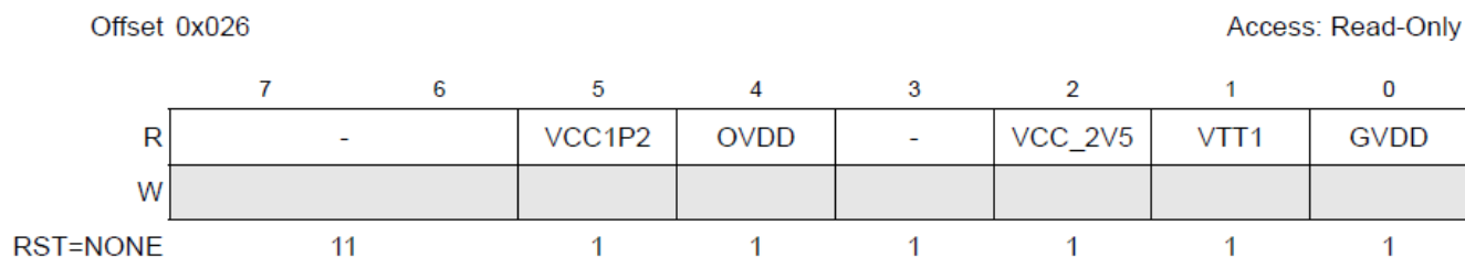
Figure 3-18. PWR_STAT2 Register
