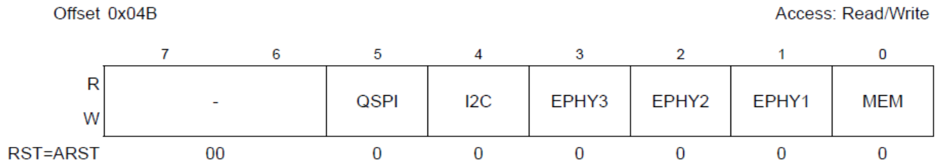
Figure 3-29. RST_MASK1 Register
