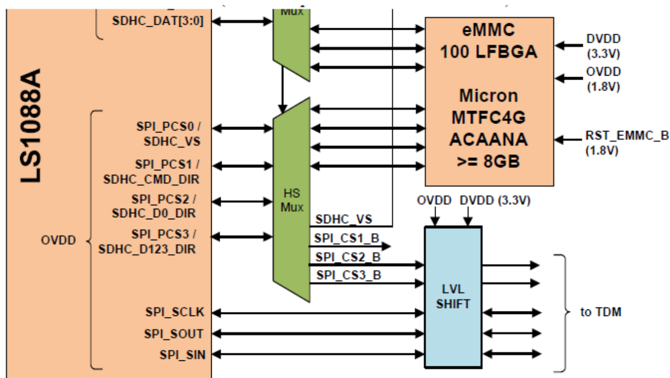
Figure 2-13. SPI interfaces
