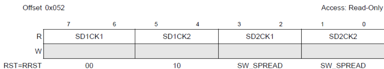
Figure 3-34. BRDCFG2 Register
