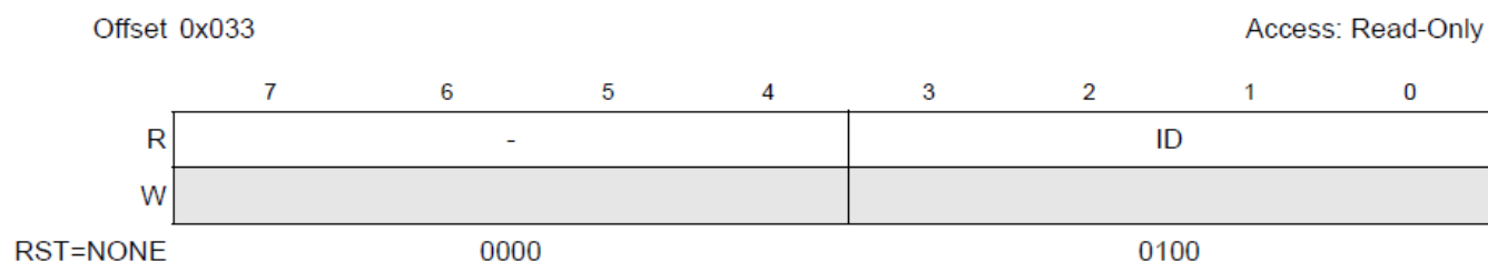
Figure 3-20. CLK_ID Register
