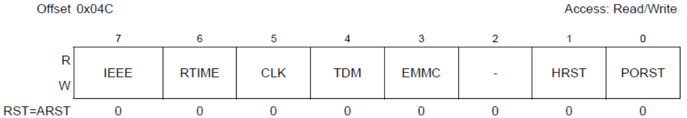
Figure 3-30. RST_MASK2 Register
