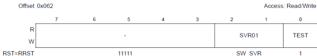
Figure 3-40. DUTCFG2 Register
