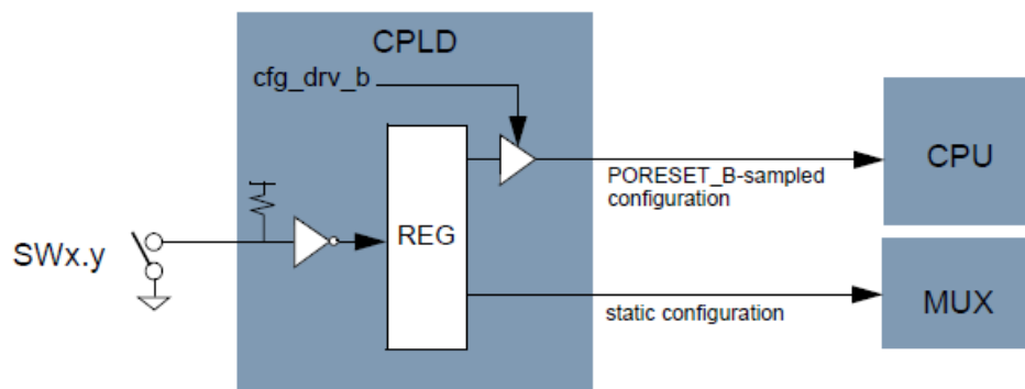
Figure 2-20. Configuration sampling
