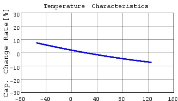
GRM21B1X1H473JA01 C-Temp. capchange, DCOV, 1
