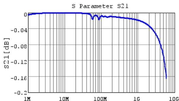
GRM21B1X1H473JA01 S21 DCOV, 20degC
