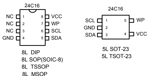
Figure 1: Package types
