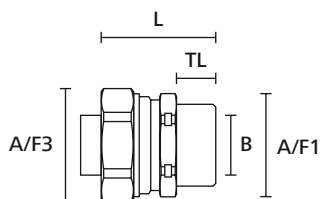
Helagaard compression fitting, straight with fixed external thread
