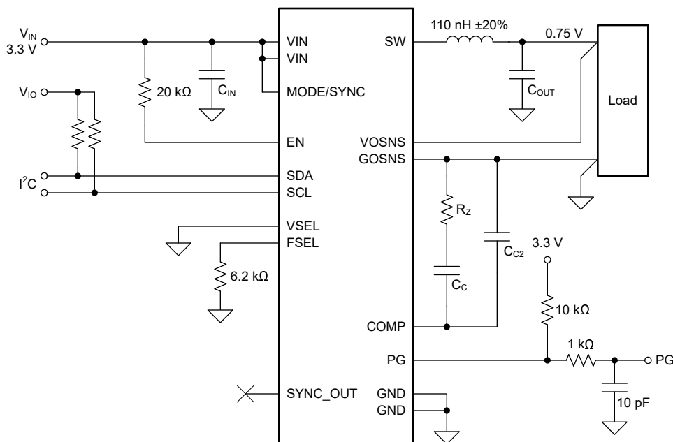
Figure 10-1. Typical Application Schematic
