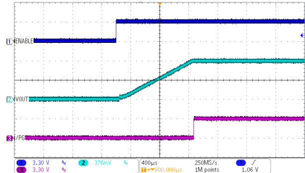
Figure 10-21. Start-Up Using the EN Pin
