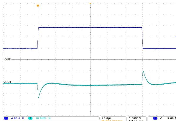
\Delta I_{OUT} = 7.5A CH1 = 50mV/A Figure 10-15. Load Transient Response
