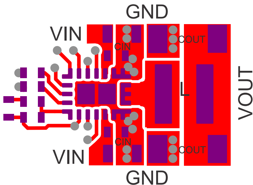
Figure 10-25. Layout Example
