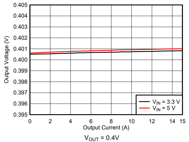
Figure 10-3. Load Regulation
