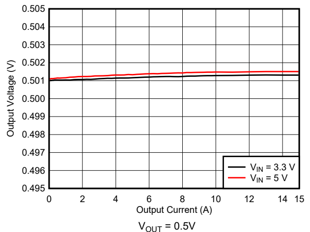
Figure 10-5. Load Regulation
