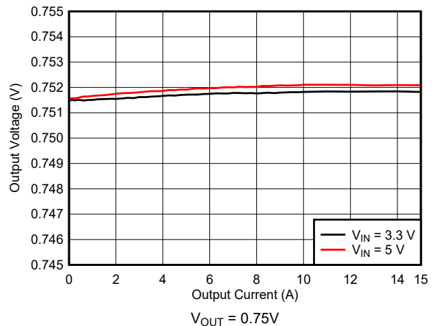
Figure 10-7. Load Regulation
