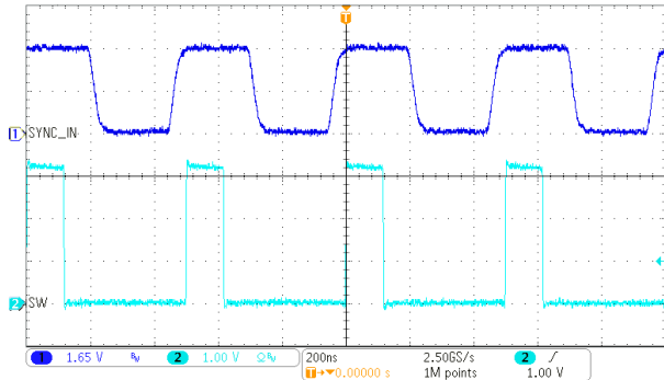
Figure 10-20. Synchronization to an External Clock
