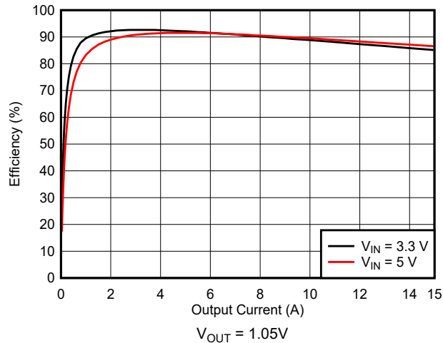
Figure 10-10. Efficiency
