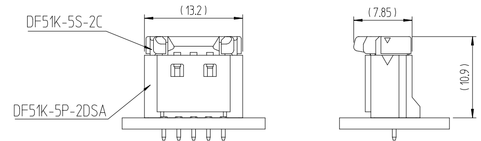
ENGAGEMENT FIGURE (2:1)
