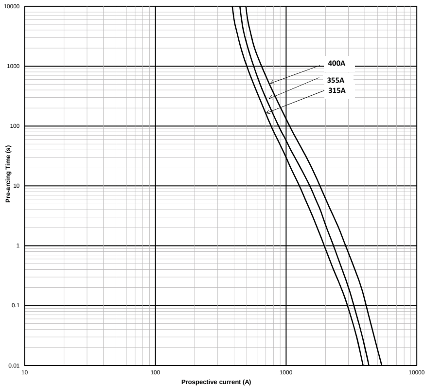
Time current-curve - Blade with bolt holes, with or without lugs
