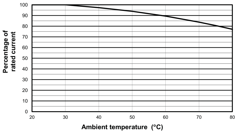
PV Array fuse link derating with temperature
