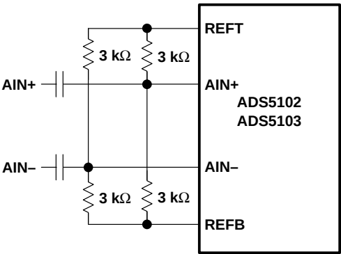
Figure 33. Driving the Analog Inputs
