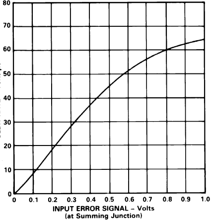
Figure 18. Slew Rate vs. Input Error Signal
