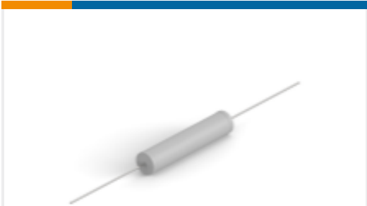
TE Part #8-2176415-9 8W STD M/OX 5% 130K
