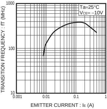
Fig.8 Transition Frequency
