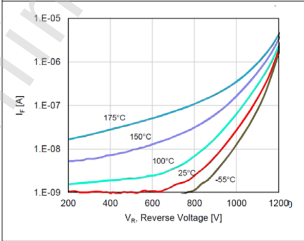
Figure 4. Reverse Characteristics
