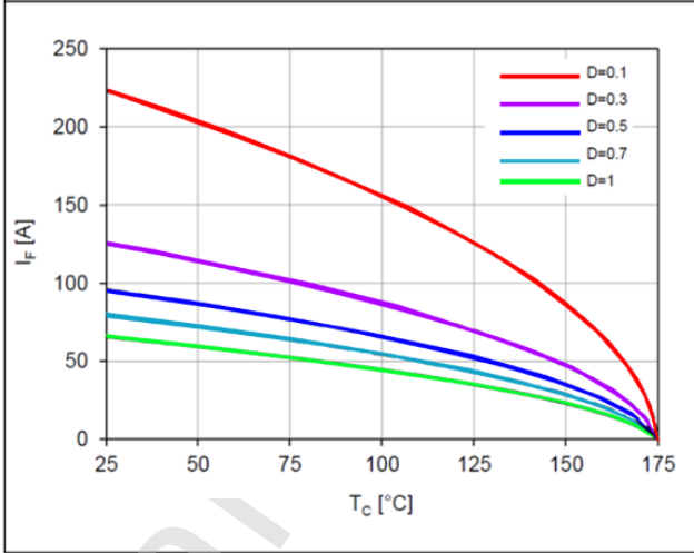
Figure 2. Current Derating
