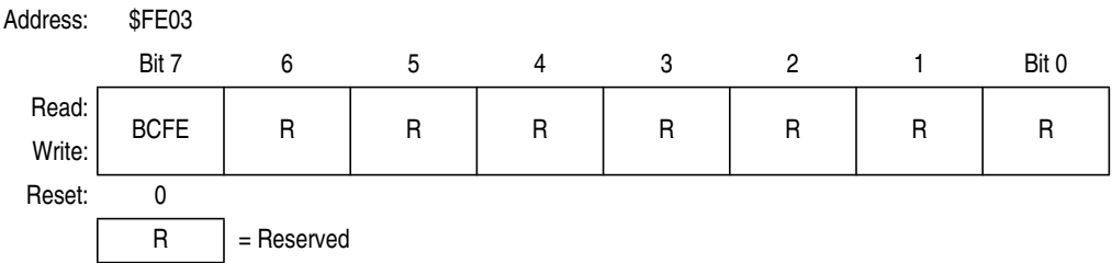
Figure 7-22. SIM Break Flag Control Register (SBFCR)
