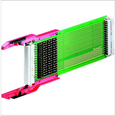
a: Measuring field for current and voltage measurement b: header for wire wrap
