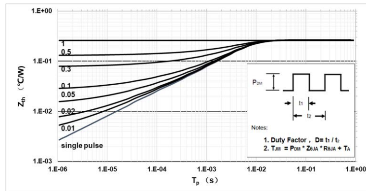
Fig 8: Transient Thermal Impandance
