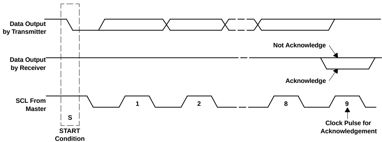
Figure 33. Acknowledge on the I²C Bus
