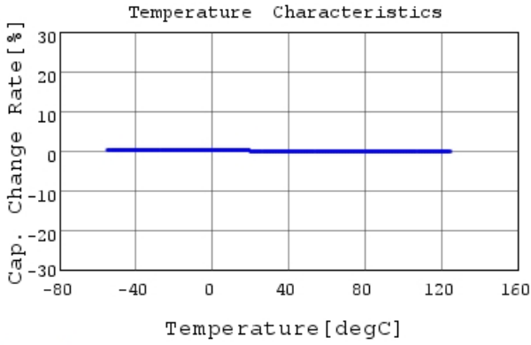
GRM1882C1H180JA01 C-Temp. capchange, DCOV, 1
