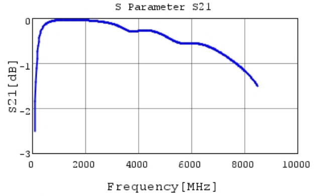
GRM1882C1H180JA01 S21 DCOV, 20degC
