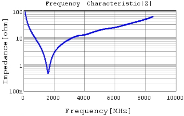
GRM1882C1H180JA01 |Z| DCOV, 20degC
