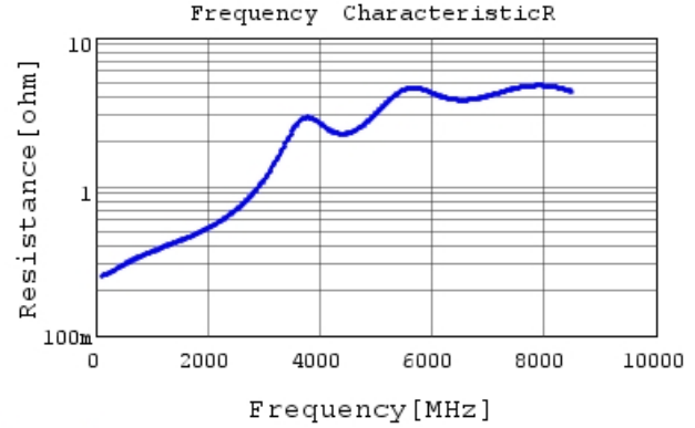
GRM1882C1H180JA01 R DCOV, 20degC
