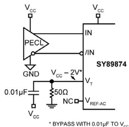
Figure 3c. DC-Coupled PECL Input Interface
