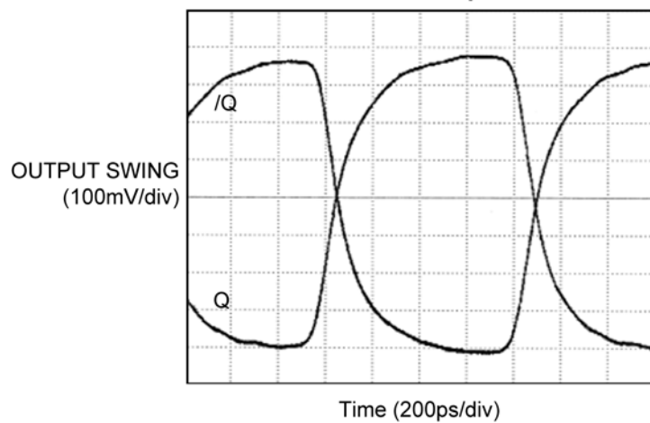
622MHz Output
