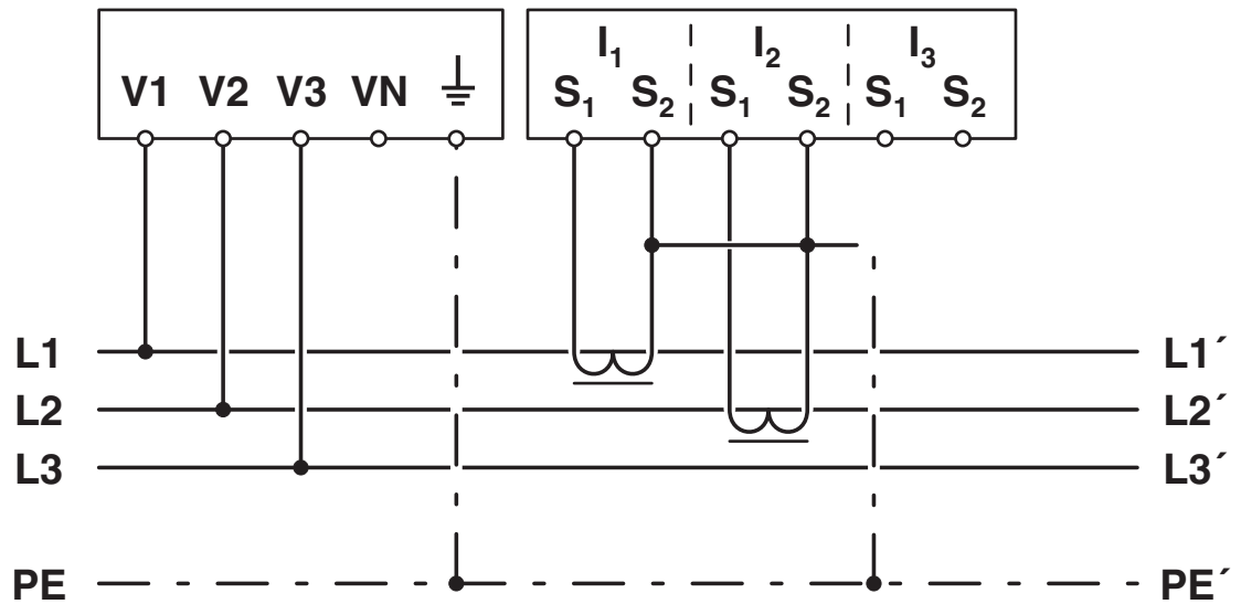
Connection diagram
