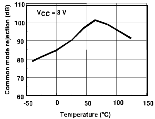
Figure 4: Common mode rejection vs. temperature ( V_{\text{CC}} = 3\text{ V} )
