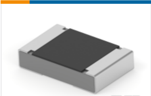
TE Part #2-2176484-3 RA73F 2A 10K 0.1% 5K RL
