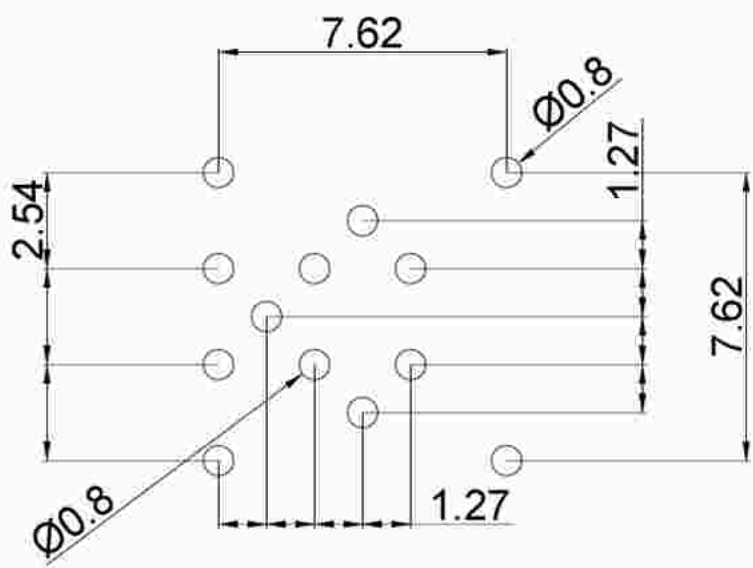
Pcb plate opening size (PCB板开孔尺寸)
