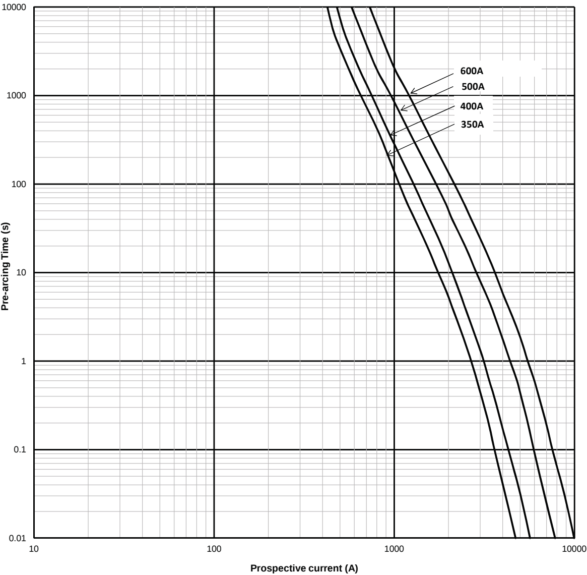
Time current curve - 1000 V d.c. - 3L - Bladed and bolted
