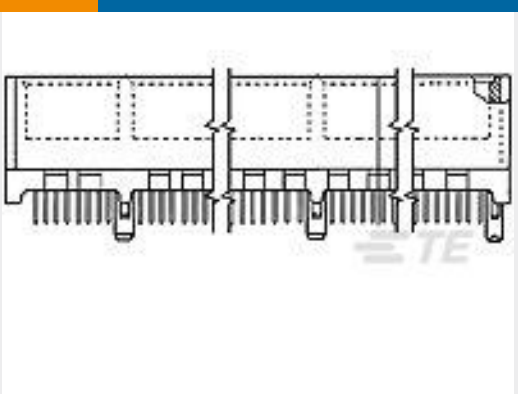
TE Part #5145165-4 STANDARD EDGE .050 SERIES 92 DUAL ASSY
