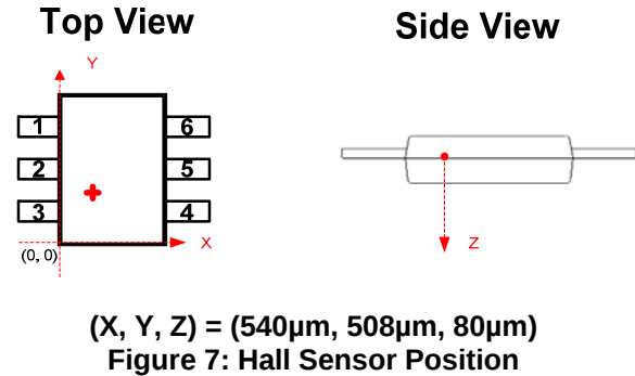
Figure 7: Hall Sensor Position
