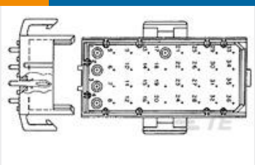
TE Part #640506-2 36P MR HDR ASSY V0
