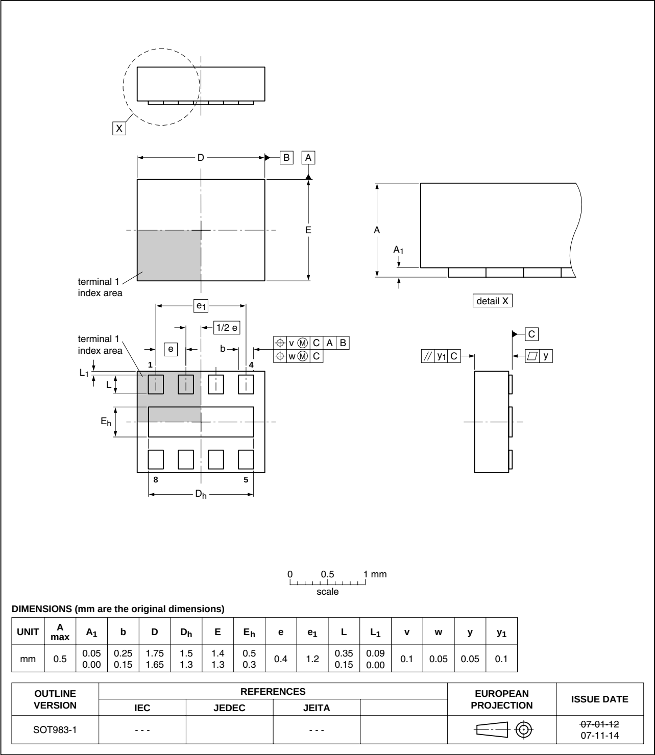
Fig 8. Package outline SOT983-1 (HXSON8U)
