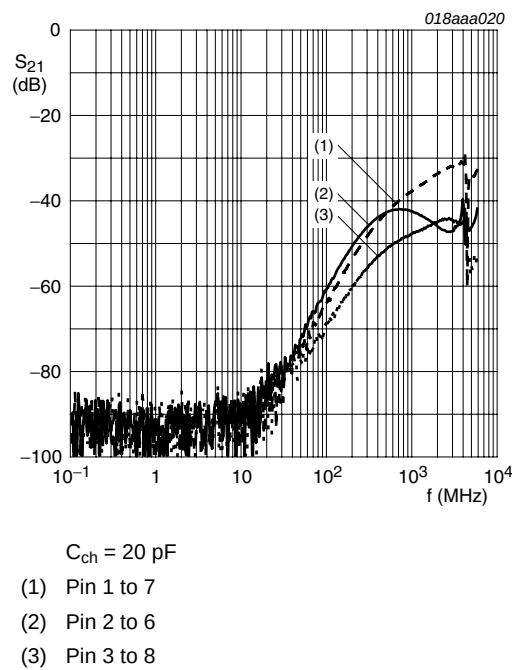
Fig 5. Crosstalk behavior for IP4264CZ8-20
