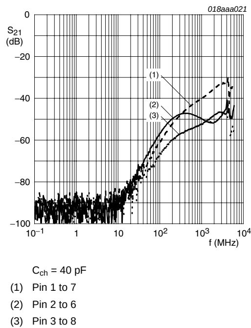
Fig 6. Crosstalk behavior for IP4264CZ8-40
