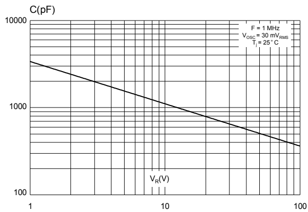
Figure 5. Junction capacitance versus reverse voltage applied (typical values, per diode)
