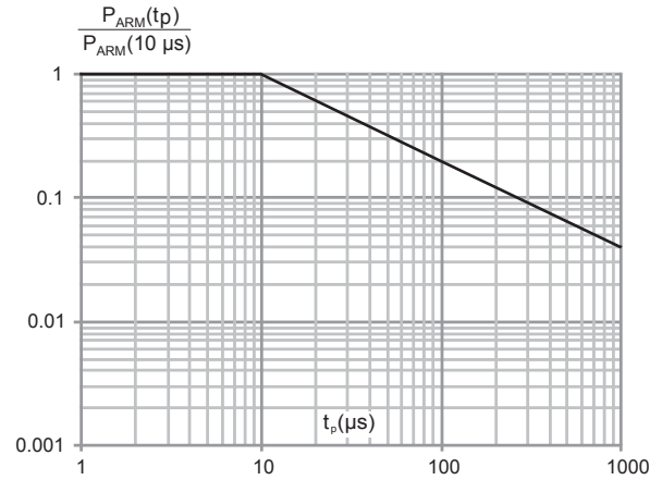
Figure 2. Normalized avalanche power derating versus pulse duration ( T_j = 125 °C)
