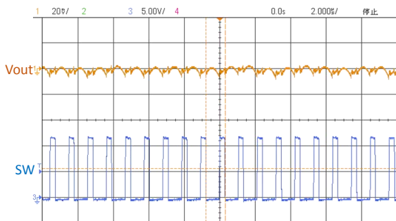
Switching Waveform at Iout = 0A (Vin=12V, Vout=3.3V)
