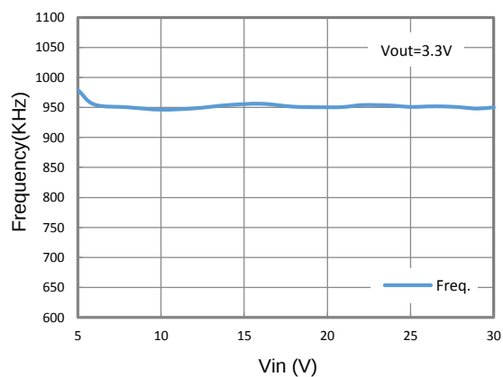
Freq. Vs. Vin
