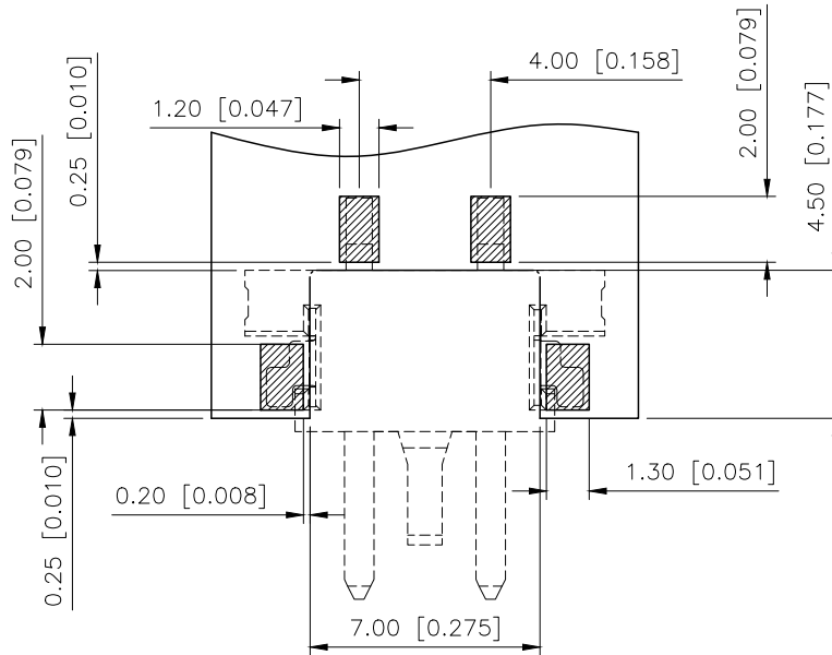
PCB_LAYOUT
