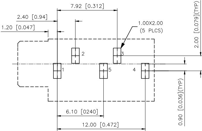
PCB Layout
