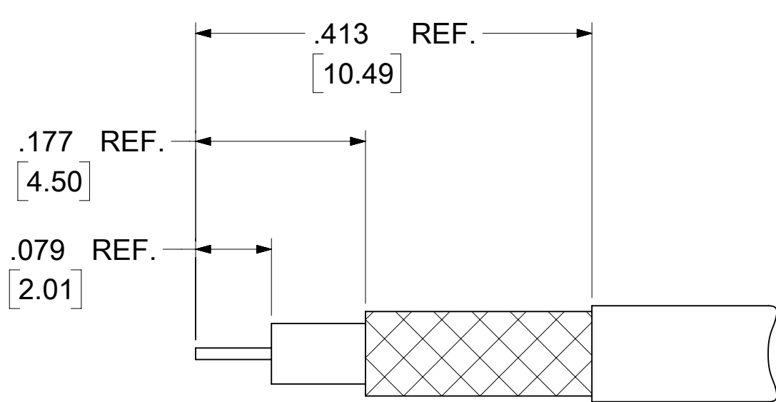
RECOMMENDED CABLE STRIP
