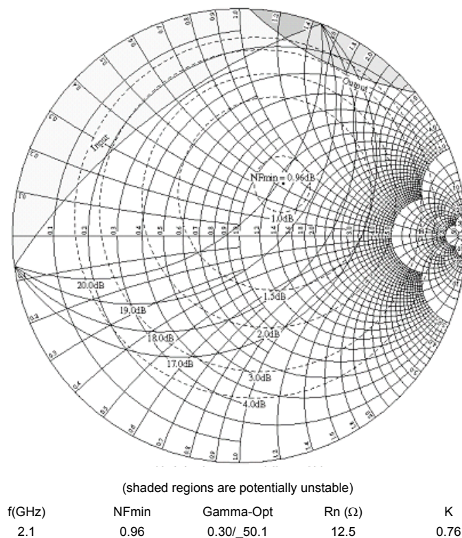
Figure 19. Constant Noise Figure and Gain Circles. 2140 MHz, Rbias =1.2 kΩ
