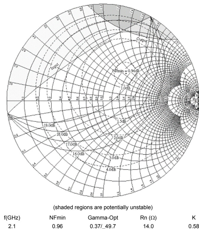
Figure 20. Constant Noise Figure and Gain Circles. 2140 MHz, Rbias =1.2 kΩ
