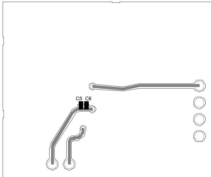
Figure 14. Back Side
