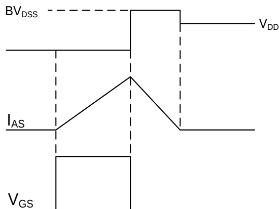
Fig.11 EAS Waveform
