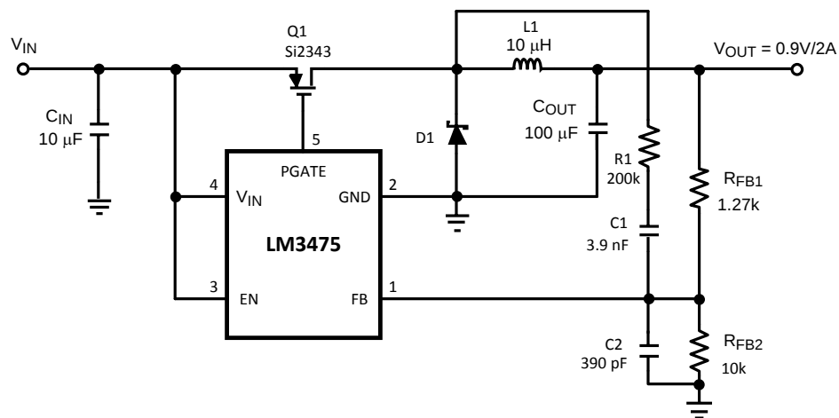
Figure 14. External Ramp
