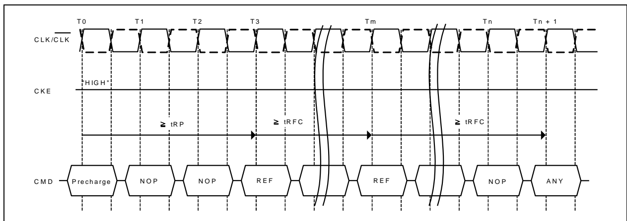
Figure 13—Refresh command
