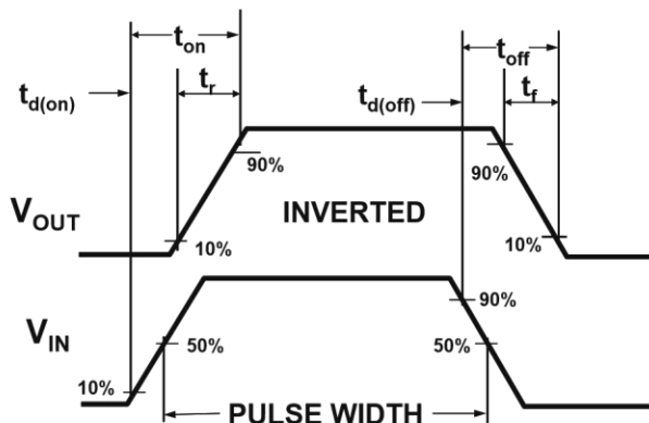
Figure 2: Switching Waveforms
