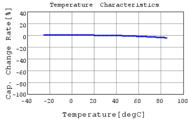
GRM022B11A101MA01 C-Temp. capchange, DC0.0V,
