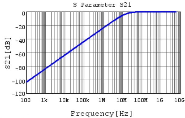
GRM022B11A101MA01 S21 DC0V,20degC
