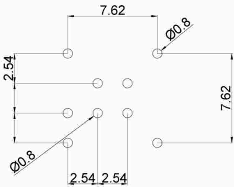
Pcb plate opening size (PCB板开孔尺寸)
