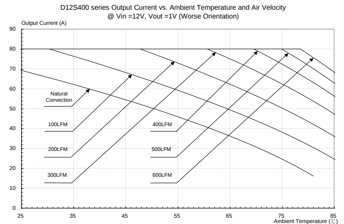
Figure 29: Output current vs. ambient temperature and air velocity @ Vin=12V, Vout=1.0V (Worst Orientation)
