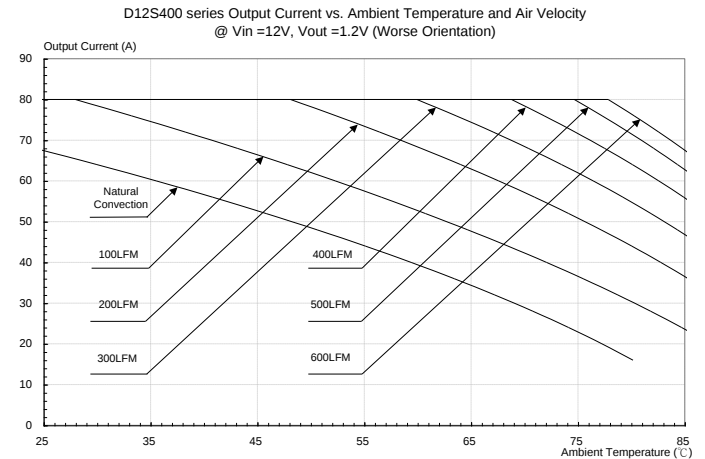
Figure 30: Output current vs. ambient temperature and air velocity @ Vin=12V, Vout=1.2V (Worst Orientation)
